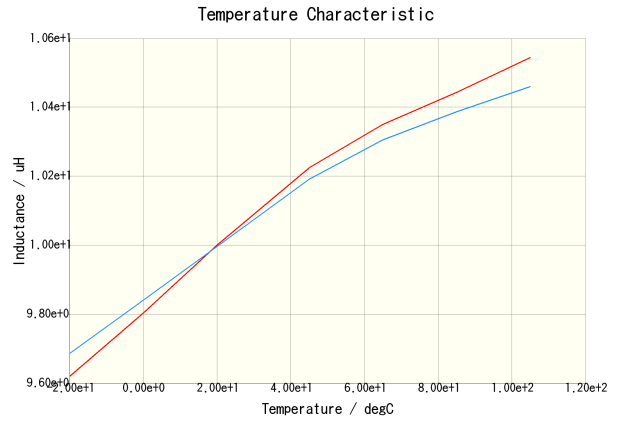
CLF7045T-100M(DC = 0A)
