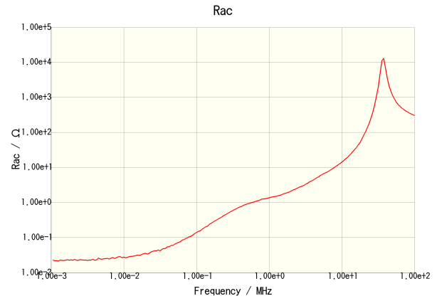
CLF7045T-100M
