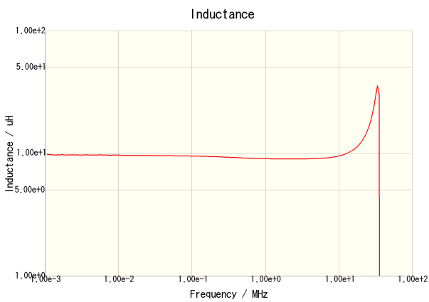
CLF7045T-100M
