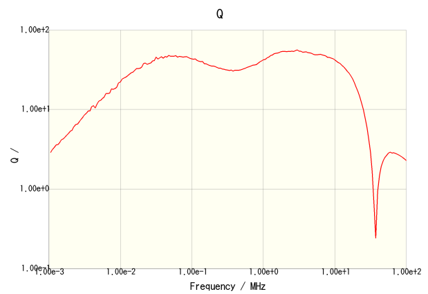
CLF7045T-100M
