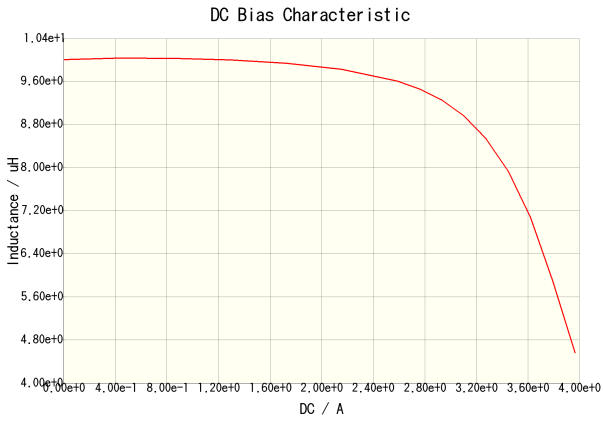
CLF7045T-100M(Amb. Temp. = 20degc)
