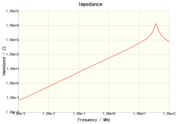
CLF7045T-100M
